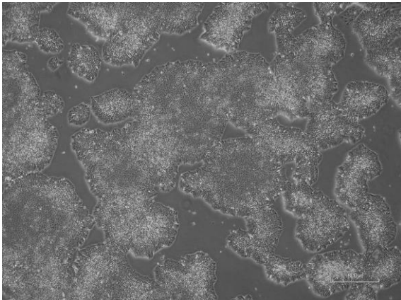
cira-jk-0136-E: passage-3
