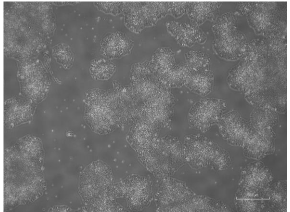
cira-jk-0136-F: passage-3
