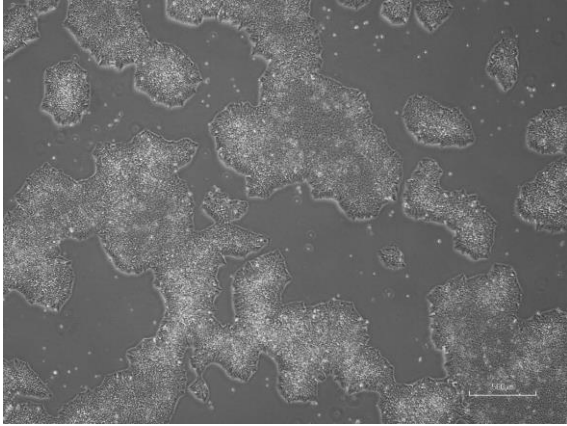
cira-jk-0136-C: passage-3
